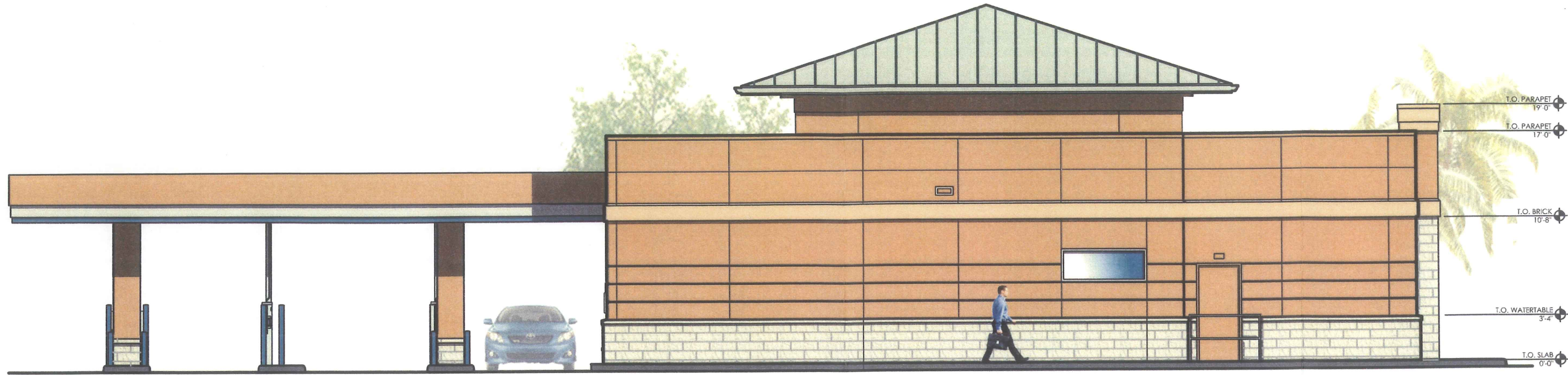
NORTH ELEVATION
